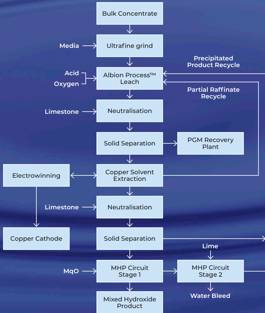
Figure 10: Flowsheet – Mixed Copper/Nickel Concentrates
